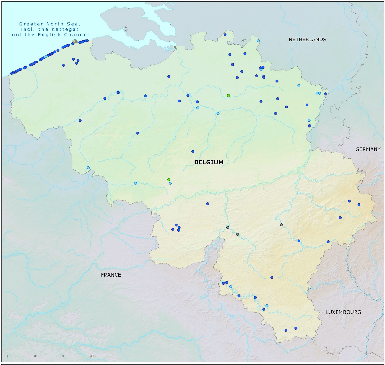
Map 1: Bathing waters reported during the 2020 bathing season in Belgium
