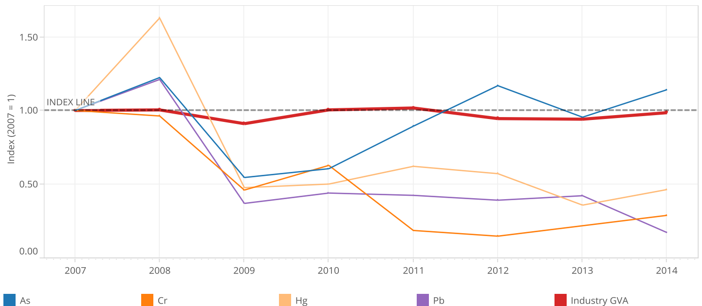
Figure 9. Industrial air pollution (based on E-PRTR data) from heavy metals versus economic growth in Portugal, 2007-2014
