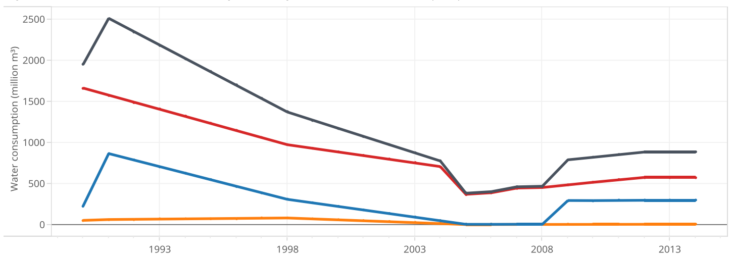
Figure 6. Evolution of industrial water usage in Portugal, in million cubic metres (Mm³), for 1990-2014
