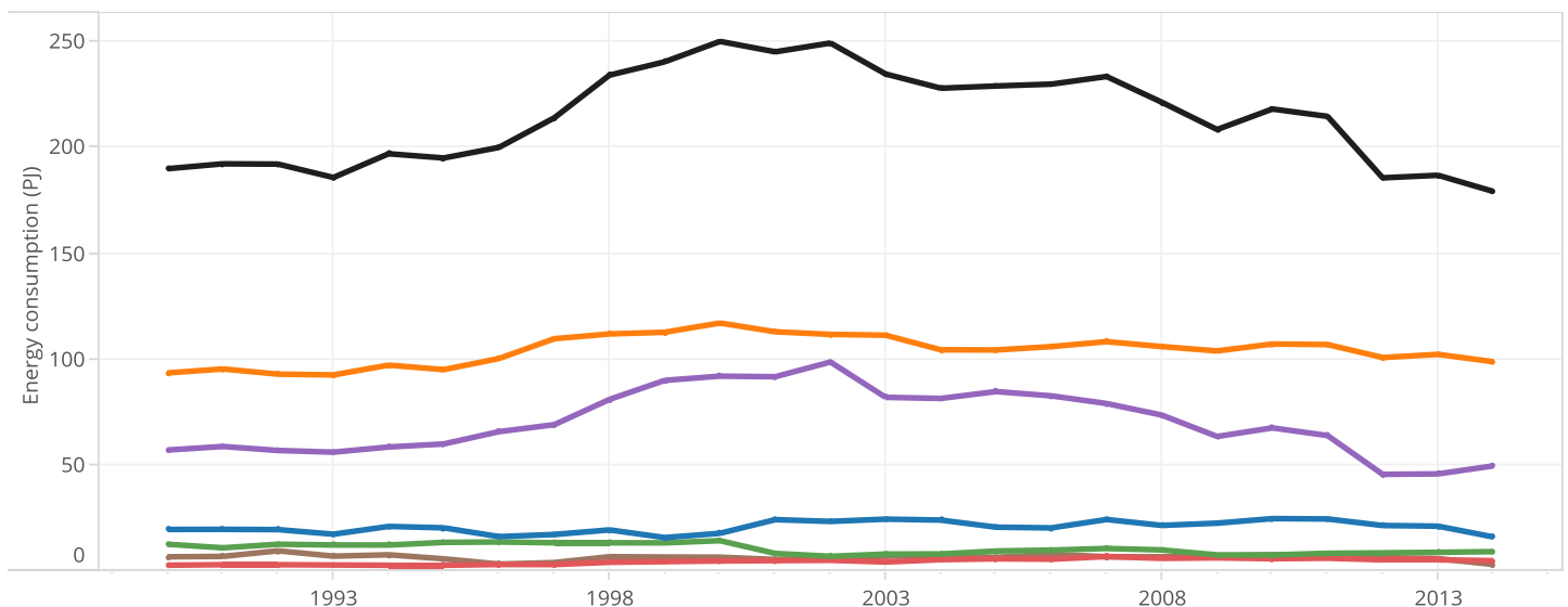
Figure 4. Evolution of the energy consumption of industry in Portugal, in petajoules (PJ), for 1990-2014
