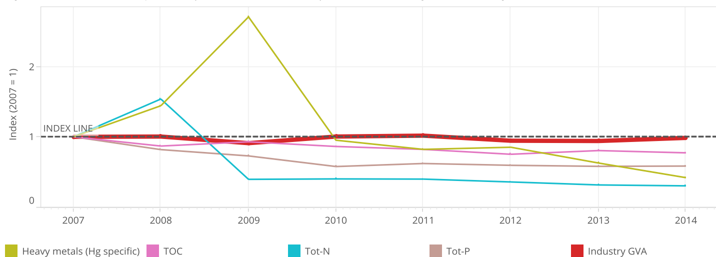
Figure 11. Industrial water pollution (based on E-PRTR data) versus economic growth in Portugal, 2007-2014
