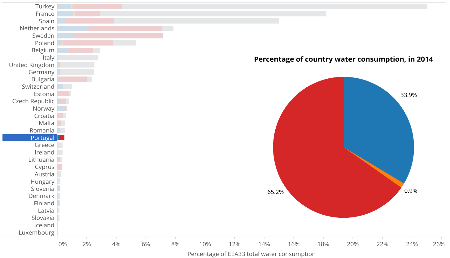
Figure 5. Water usage by industry as a percentage of EEA33 water usage, and within Portugal, in 2014
