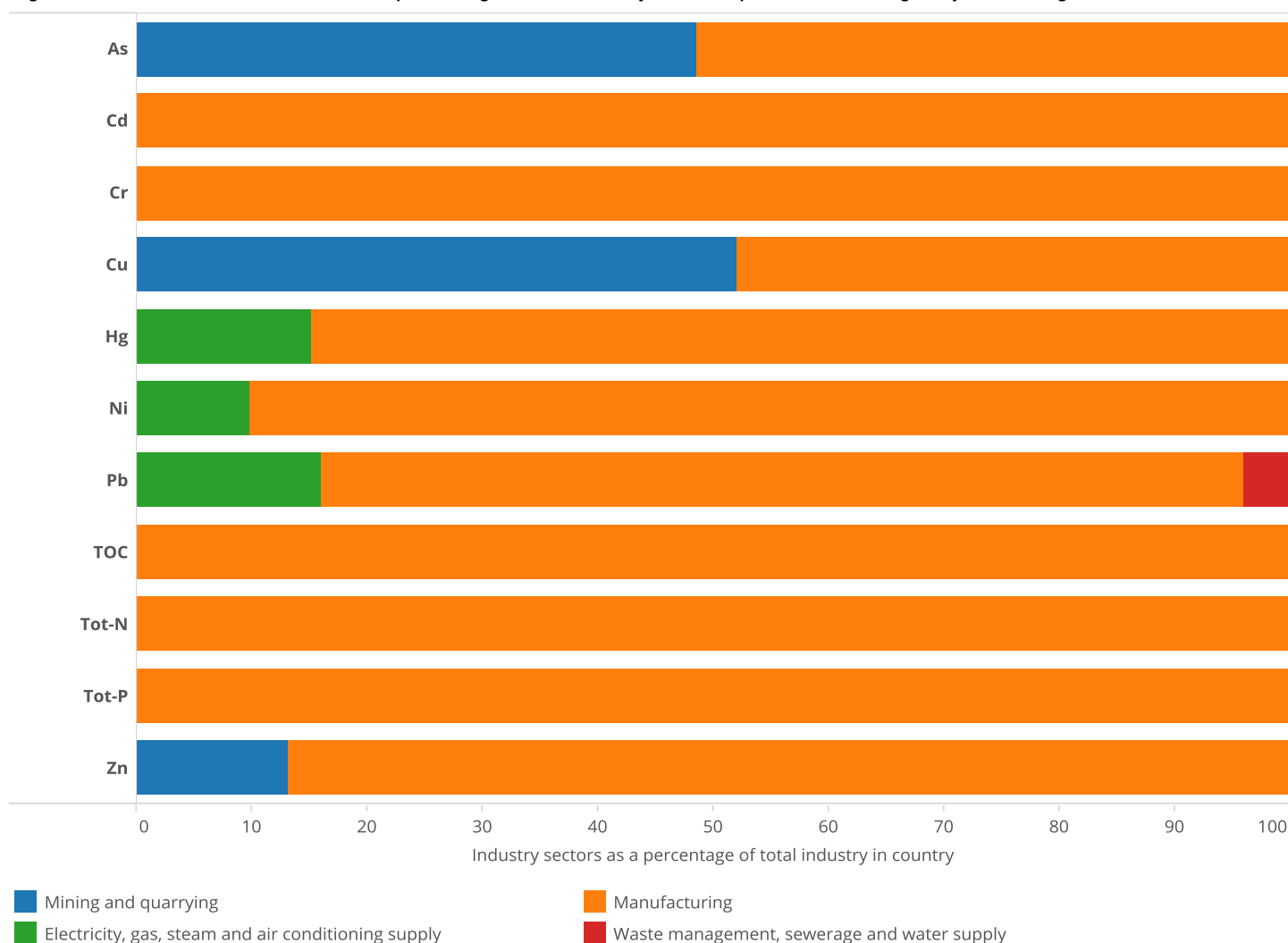
Figure 10. Industrial water releases as a percentage of total country E-PRTR pollution in Portugal, by sector origins, in 2014
