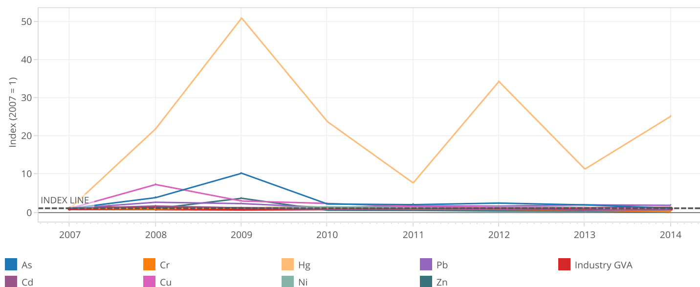
Figure 12. Industrial water pollution (based on E-PRTR data), from heavy metals, versus economic growth in Portugal, 2007-2014
