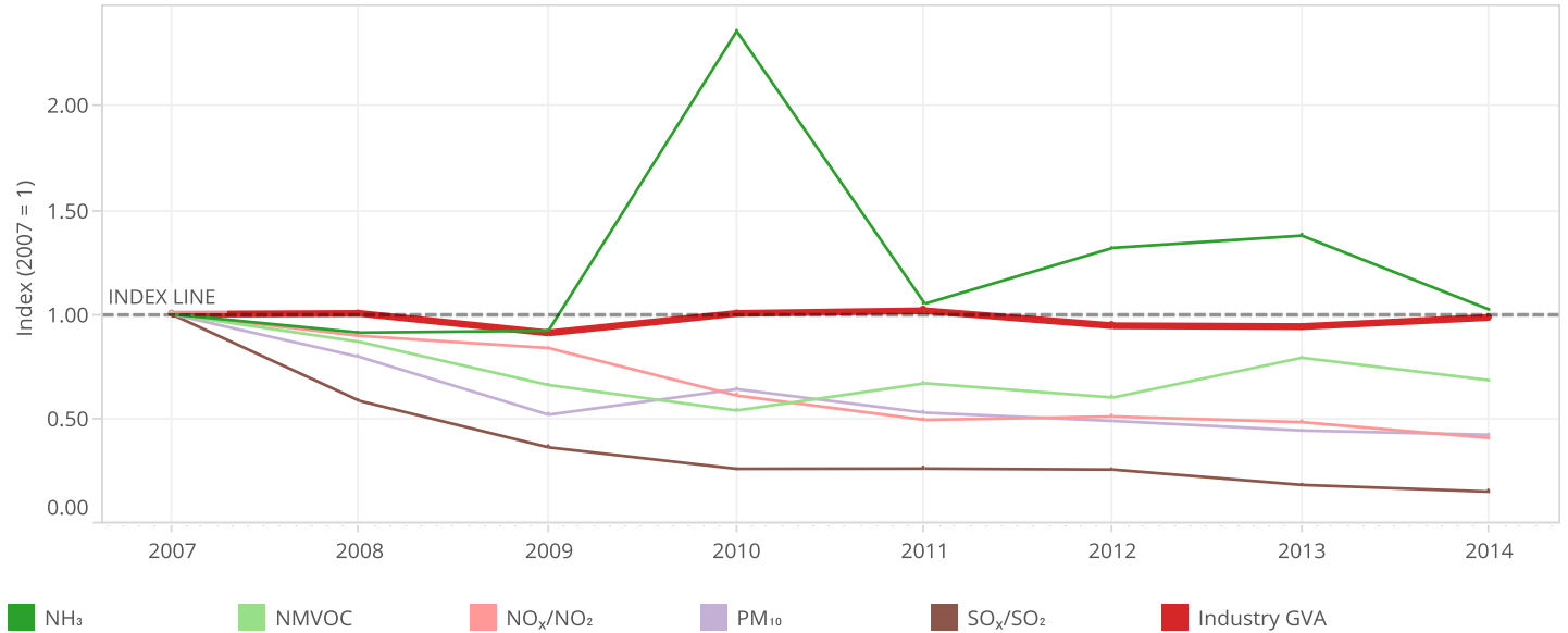
Figure 8. Industrial air pollution (based on E-PRTR data) from non-heavy metals versus economic growth in Portugal, 2007-2014
