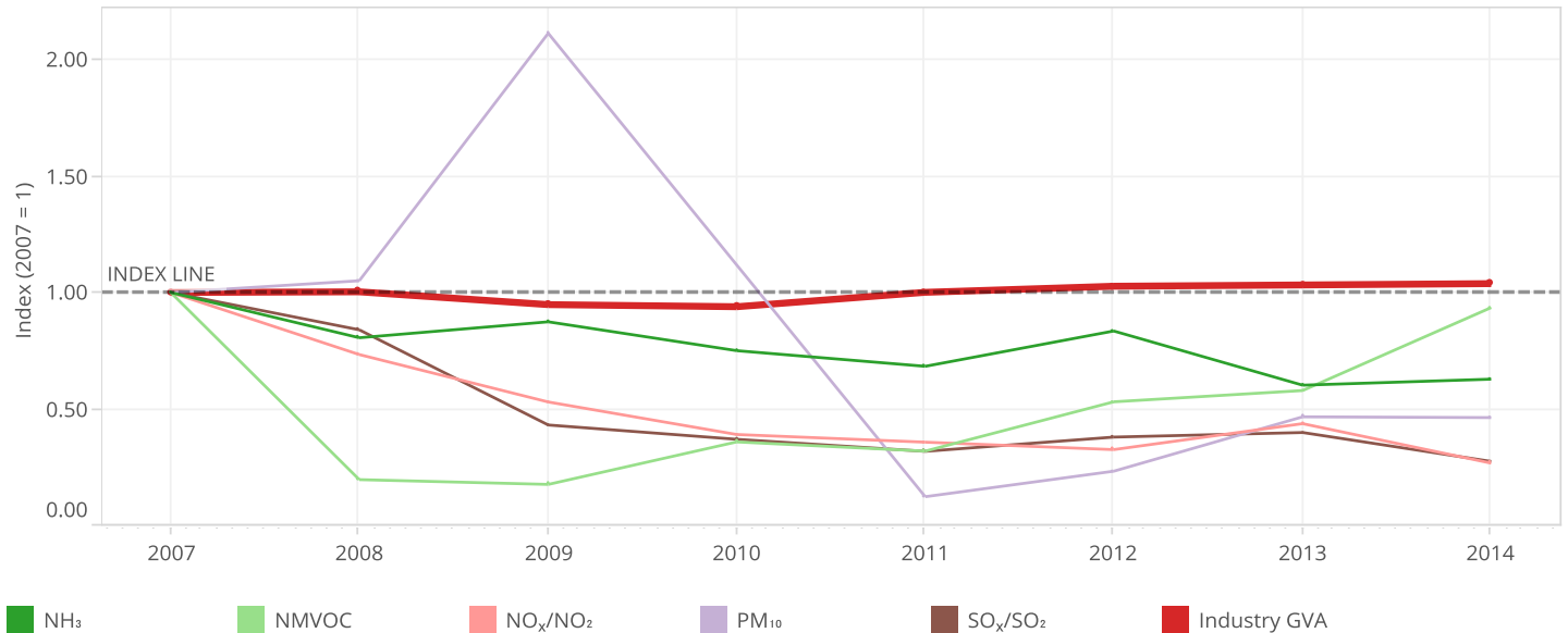
Figure 8. Industrial air pollution (based on E-PRTR data) from non-heavy metals versus economic growth in Denmark, 2007-2014
