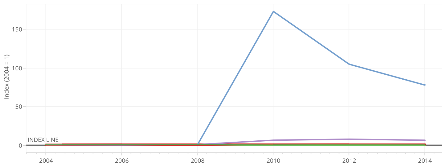
Figure 17. Decoupling of industrial hazardous waste in Denmark, 2004-2014 (latest years available)
