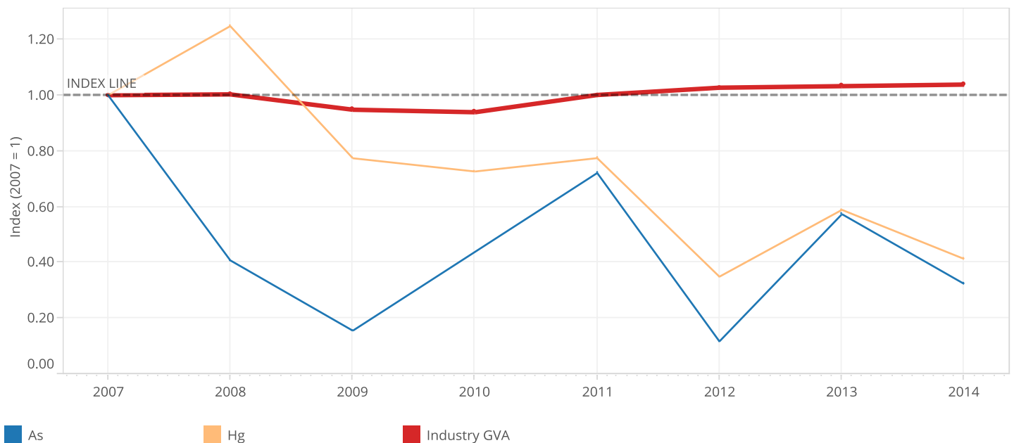
Figure 9. Industrial air pollution (based on E-PRTR data) from heavy metals versus economic growth in Denmark, 2007-2014
