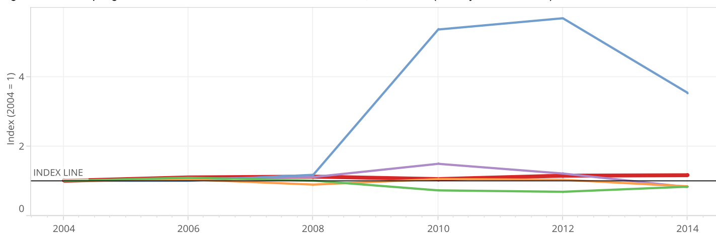
Figure 16. Decoupling of industrial non-hazardous waste in Denmark, 2004-2014 (latest years available)
