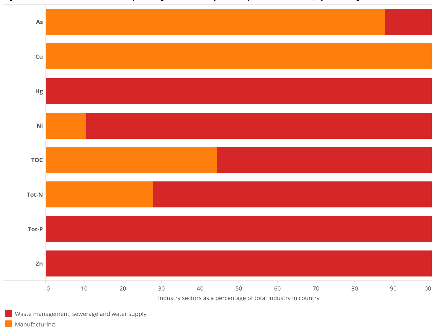
Figure 10. Industrial water releases as a percentage of total country E-PRTR pollution in Denmark, by sector origins, in 2014
