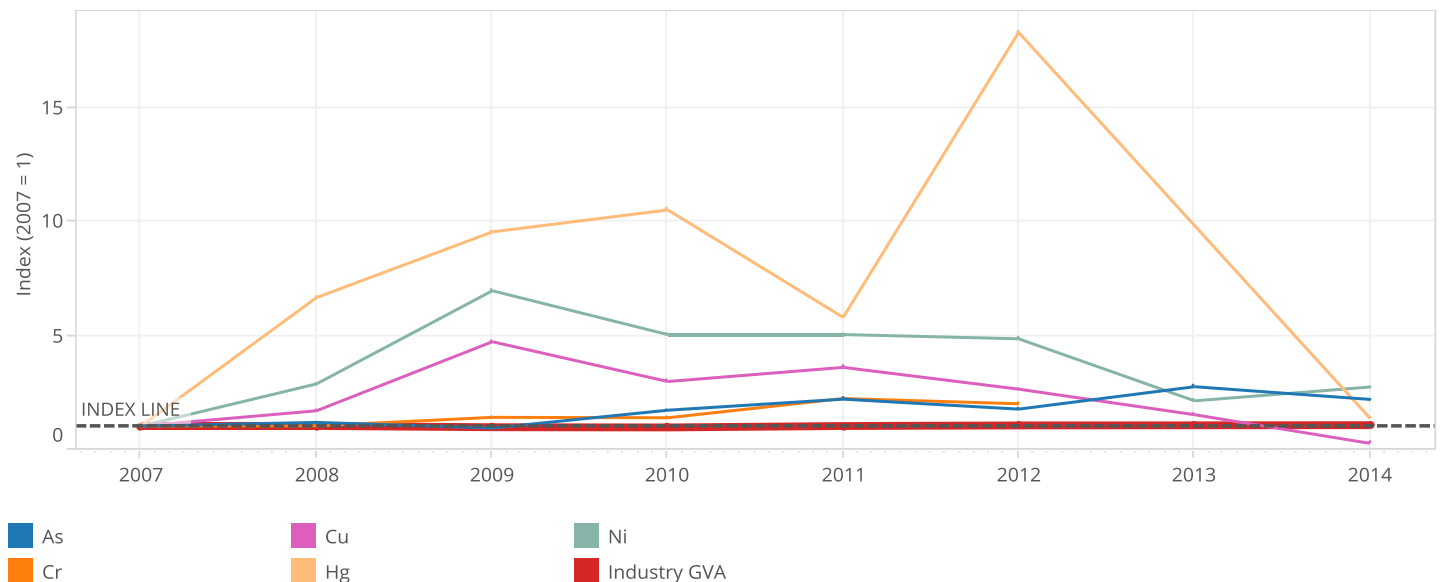
Figure 12. Industrial water pollution (based on E-PRTR data), from heavy metals, versus economic growth in Denmark, 2007-2014
