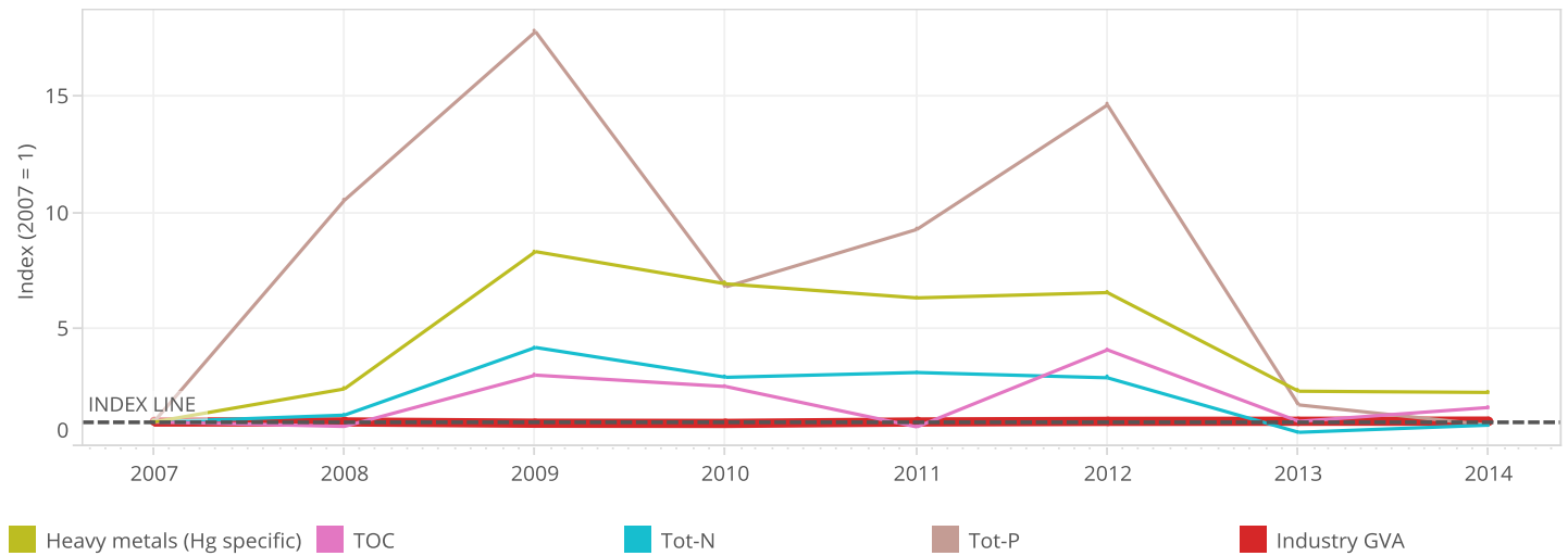
Figure 11. Industrial water pollution (based on E-PRTR data) versus economic growth in Denmark, 2007-2014
