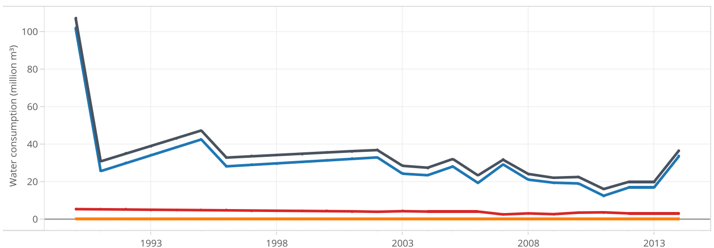
Figure 6. Evolution of industrial water usage in Denmark, in million cubic metres (Mm³), for 1990-2014
