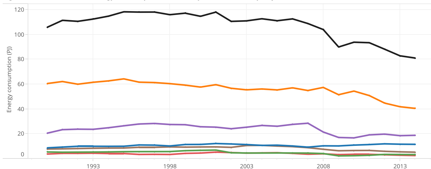
Figure 4. Evolution of the energy consumption of industry in Denmark, in petajoules (PJ), for 1990-2014
