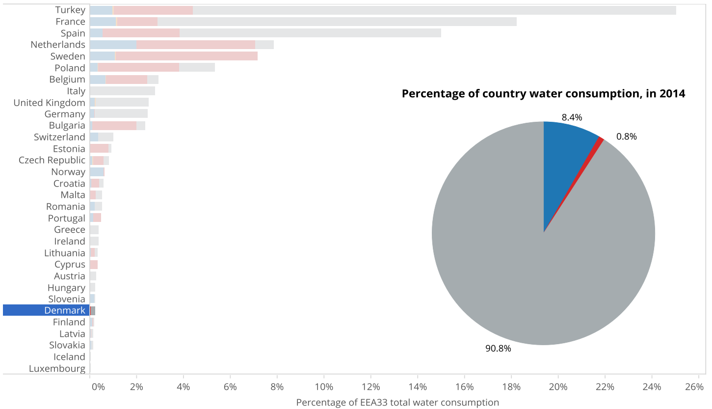
Figure 5. Water usage by industry as a percentage of EEA33 water usage, and within Denmark, in 2014
