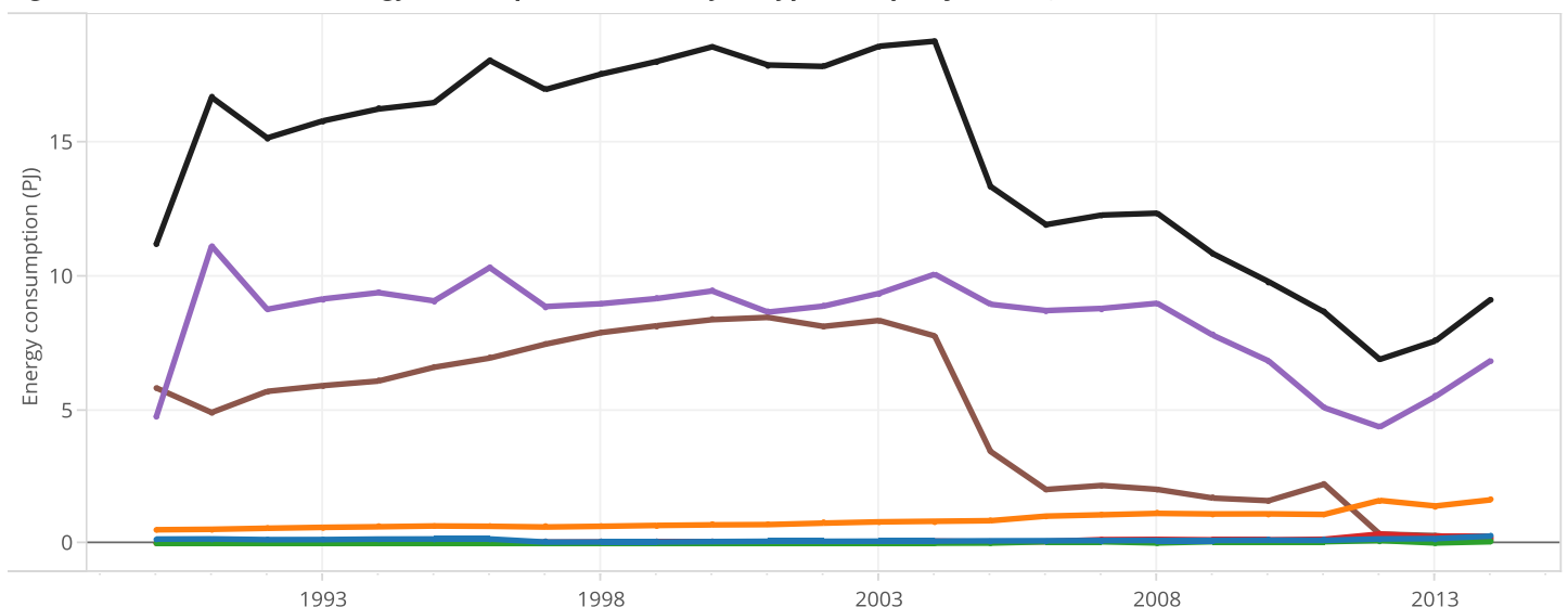
Figure 4. Evolution of the energy consumption of industry in Cyprus, in petajoules (PJ), for 1990-2014
