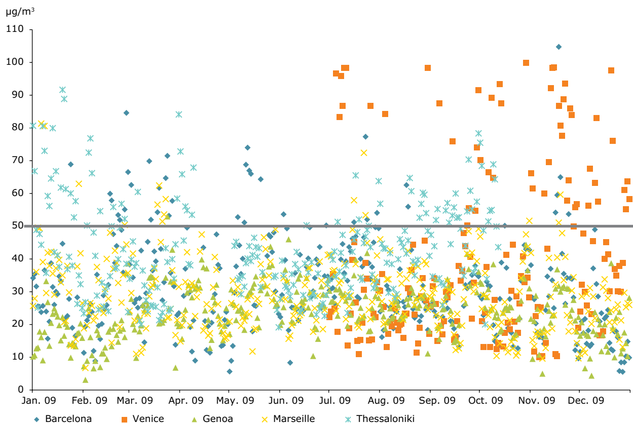
Figure 5.2 Daily variation (in \mu\text{g}/\text{m}^3 ) of \text{PM}_{10} concentrations in 2009
