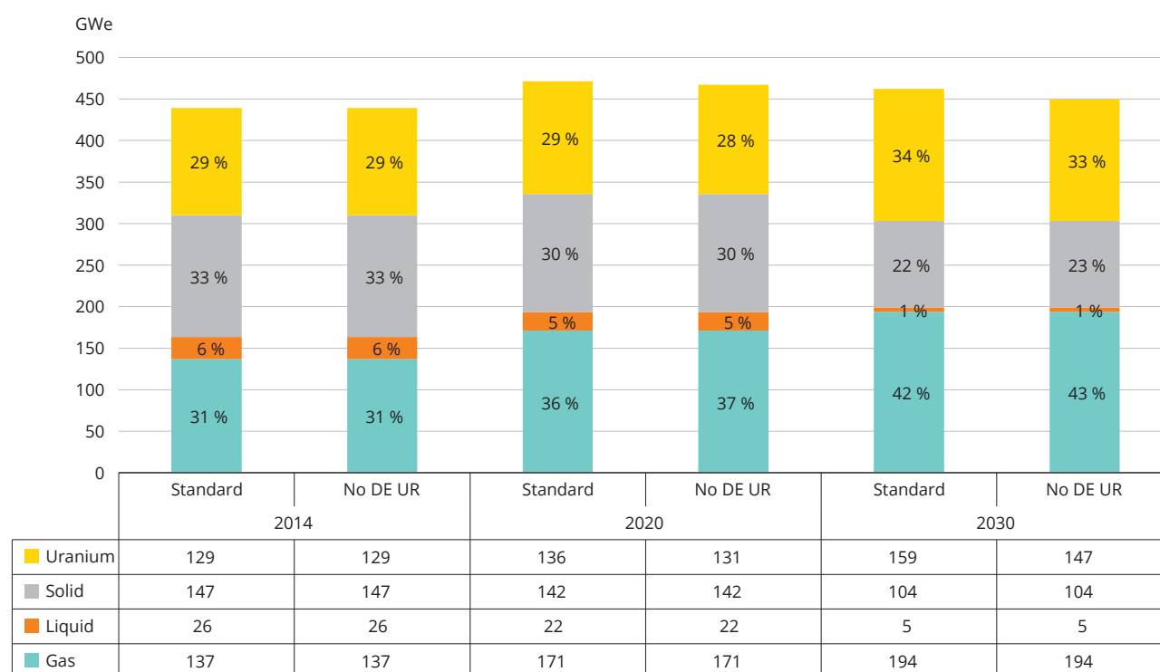
Figure A1.9 Comparison of extended (EXT) lifetimes variant with an extended (EXT) lifetimes variant and accelerated German nuclear decommissioning lifetimes
