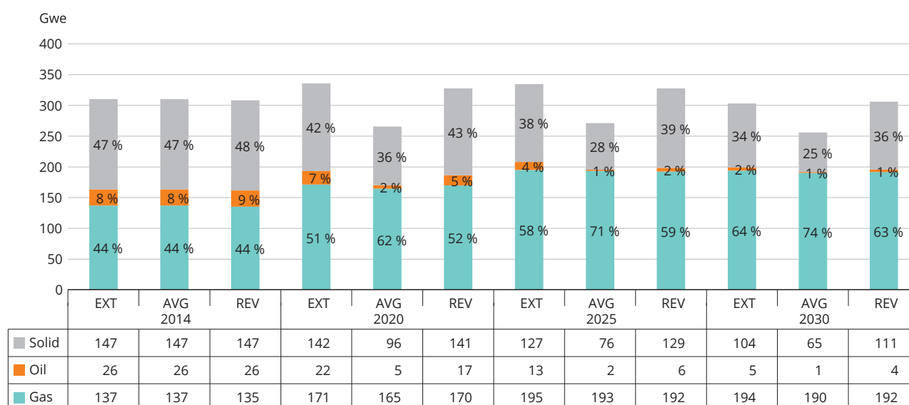
Figure 3.11 Installed capacity expected to remain operational up to 2030 by fuel type in the EU-28
