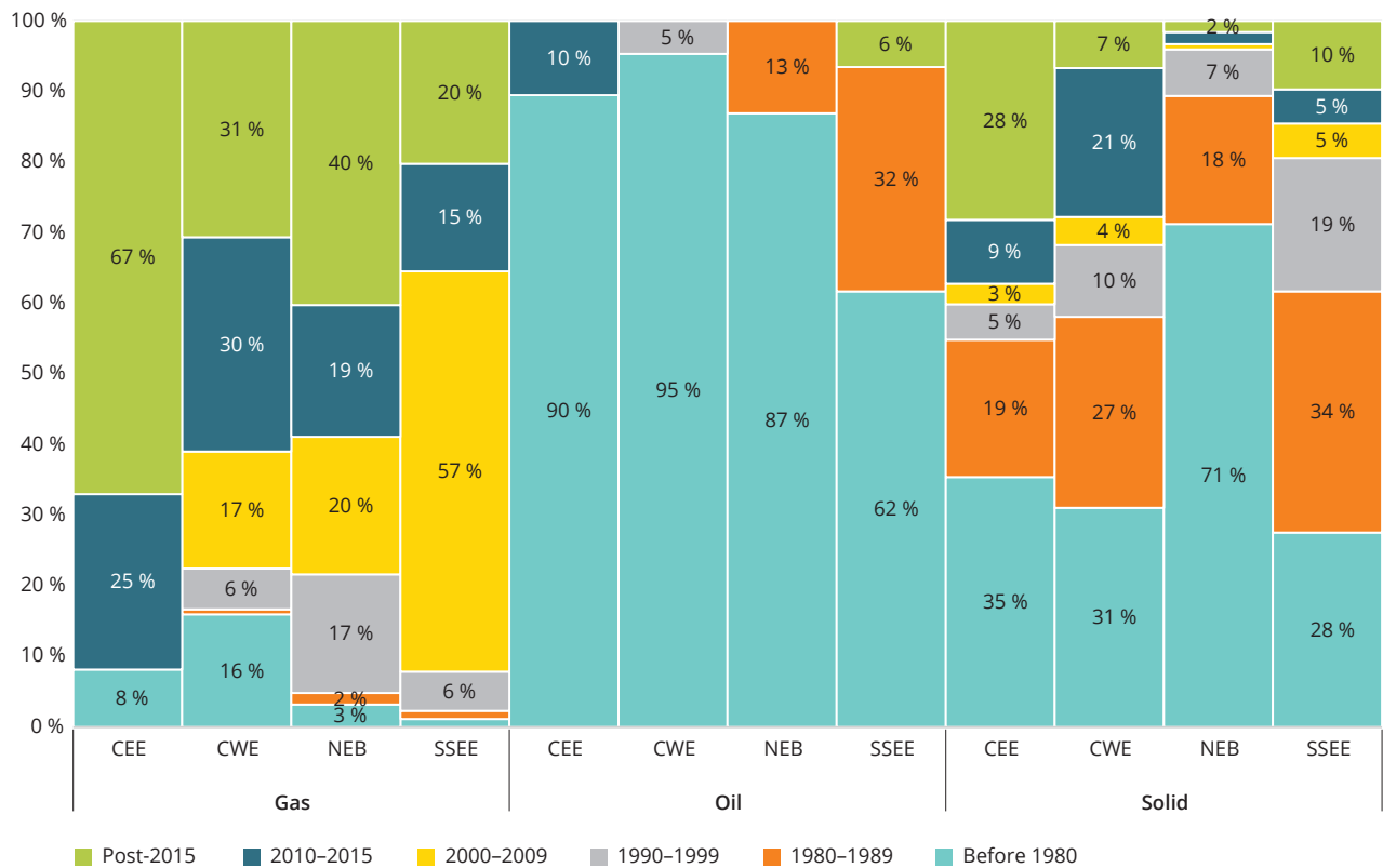
Figure ES.2 Age of capacity by fossil fuel type, by region
