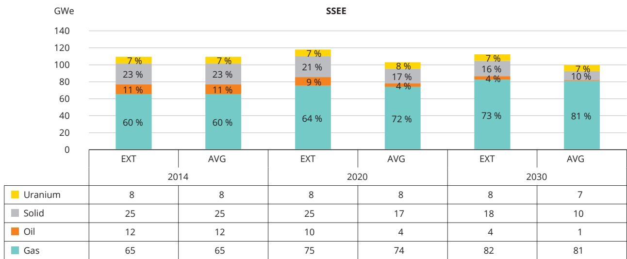
Figure A1.7 Installed capacity in south and south-eastern Europe
