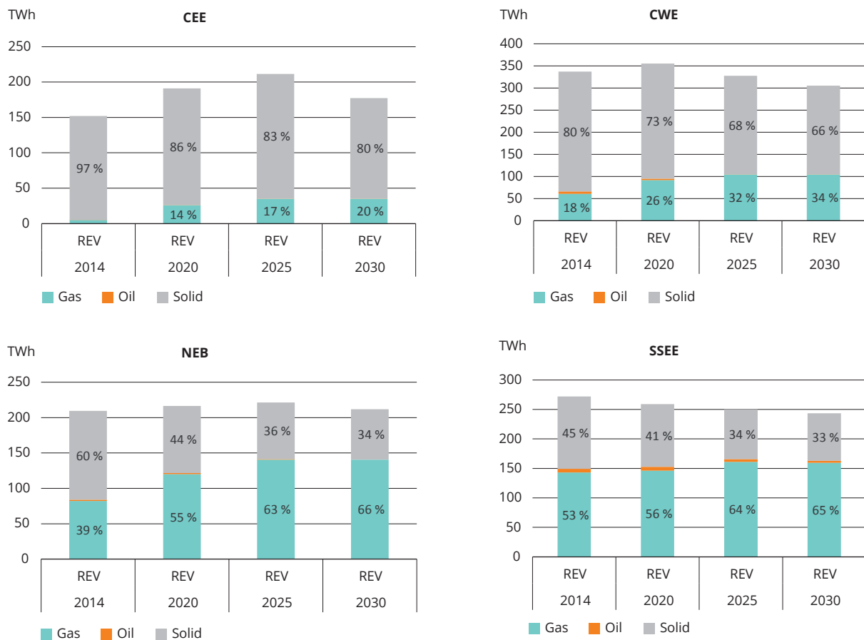
Figure 3.12 Regional power mix profiles (REV pathway)
