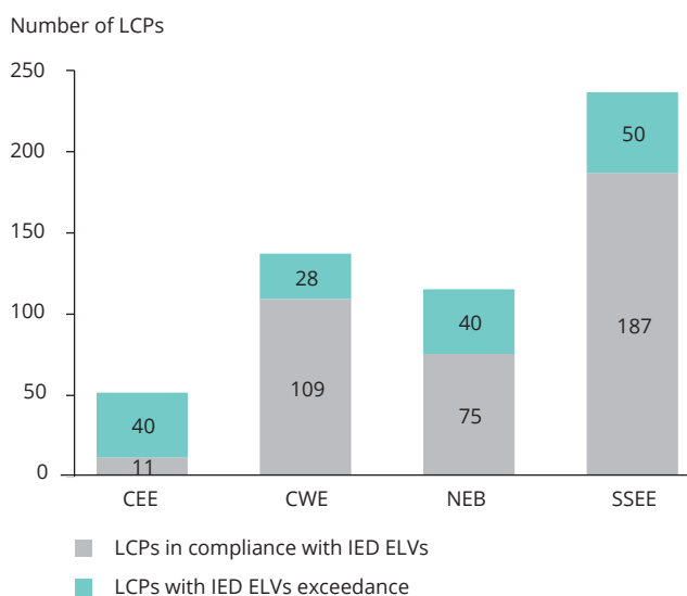
Figure 3.5 Number of LCPs with and without IED ELV exceedances, by region
