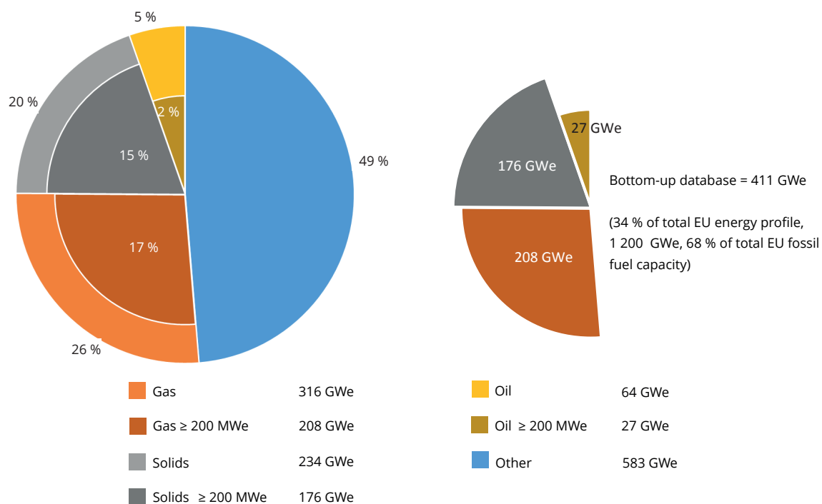
Figure 1.1 Representation of capacity assessed under this study, versus all EU power capacity
