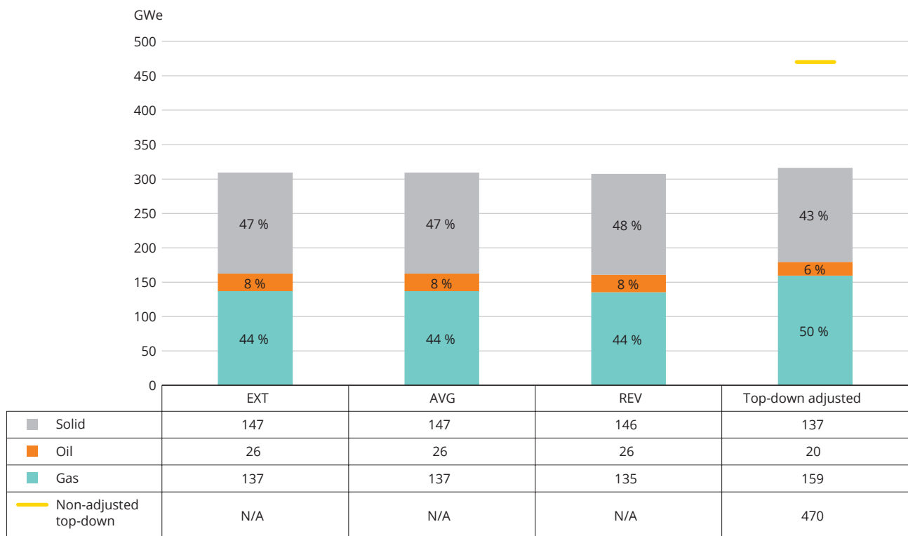
Figure 2.7 Comparison of currently installed EU-27 capacity profiles, 2014/2015, by fuel type (GWe)
