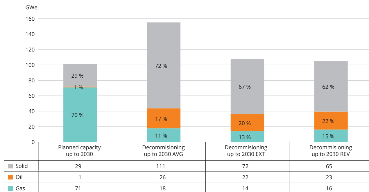
Figure 3.10 Comparison between the expected decommissioning of units and planned units up to 2030 (GWe)
