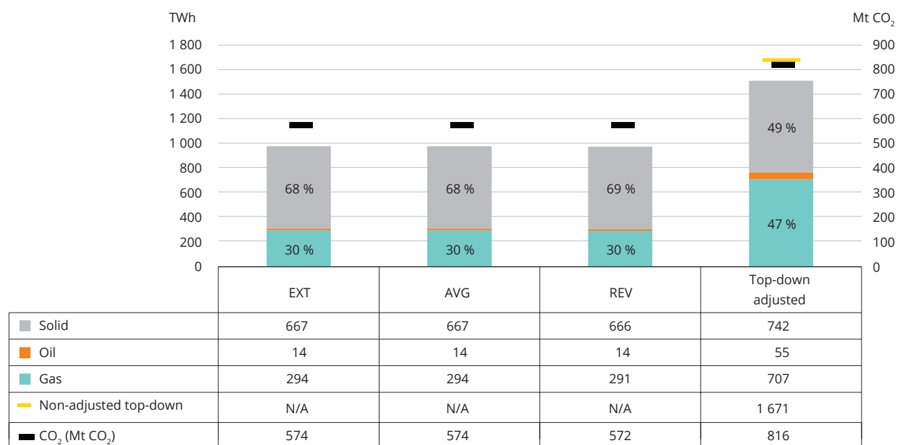
Figure 2.9 Comparison of current EU-27 electricity generation profiles by fuel type (TWh) and carbon dioxide emissions (Mt CO 2 ), 2014/2015
