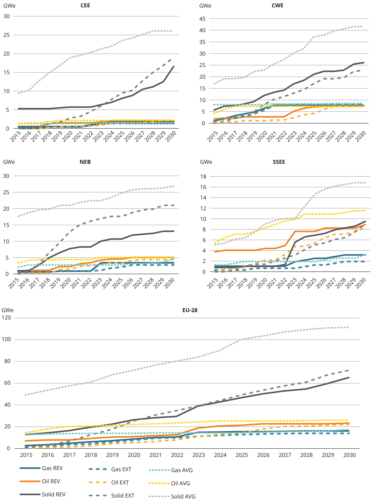
Figure 3.9 EXT and REV decommissioning pathways (by region and fuel, covering EU-28 capacity up to 2030)
