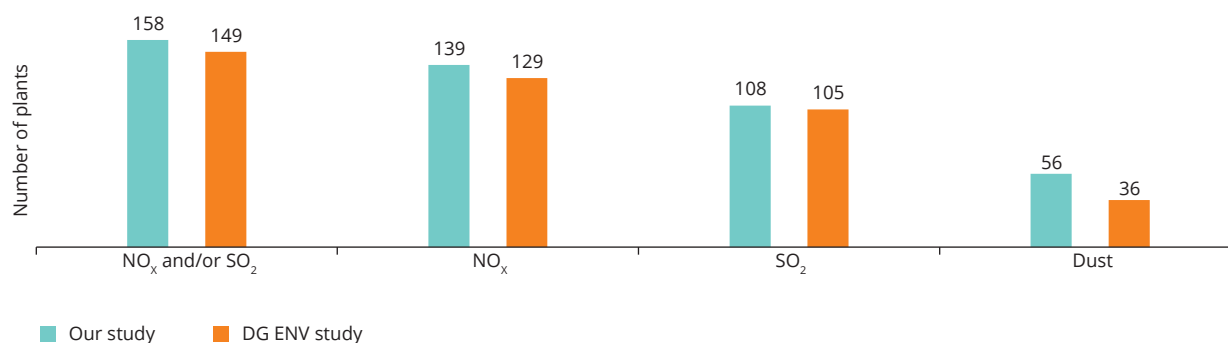
Figure 3.2 Number of LCPs exceeding IED ELVs for NO x , SO 2 and dust
