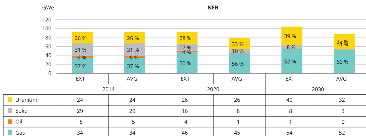
Figure A1.6 Installed capacity in northern Europe and the Baltics (GWe)
