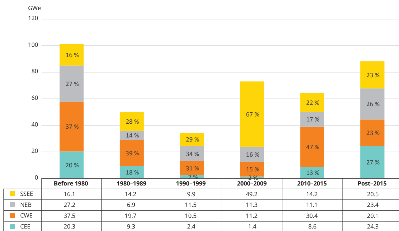
Figure 2.4 Total expected regional capacity profile by year of construction (fossil fuel units ≥ 200 MWe)
