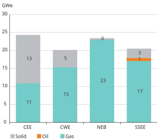
Figure ES.3 New fossil fuel capacity post-2015, by region in the EU-28
