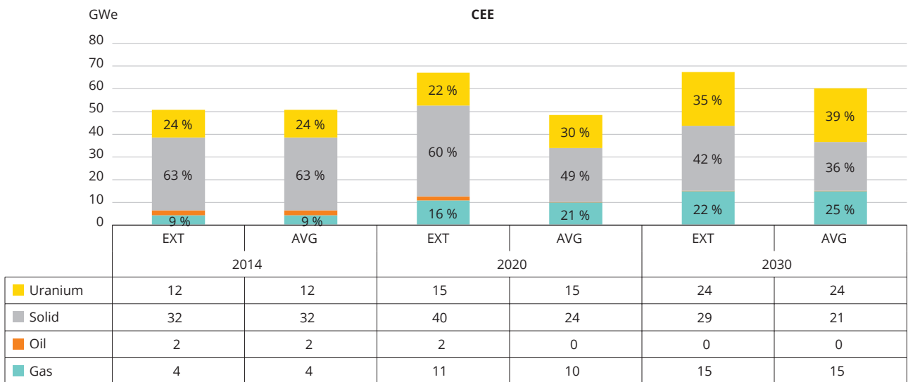
Figure A1.4 Installed capacity in central-eastern Europe (GWe)
