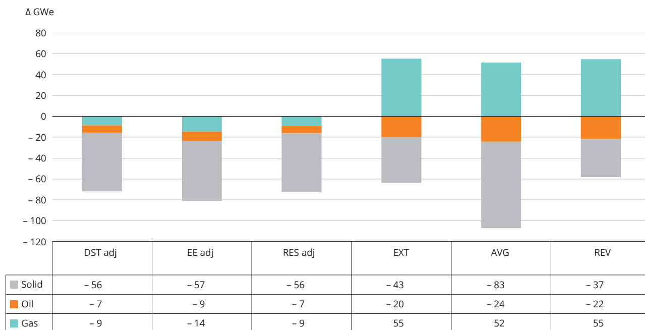
Figure 4.4 Capacity change from 2015 to 2030 by fuel type and scenario in the EU-27 (Δ GWe)
