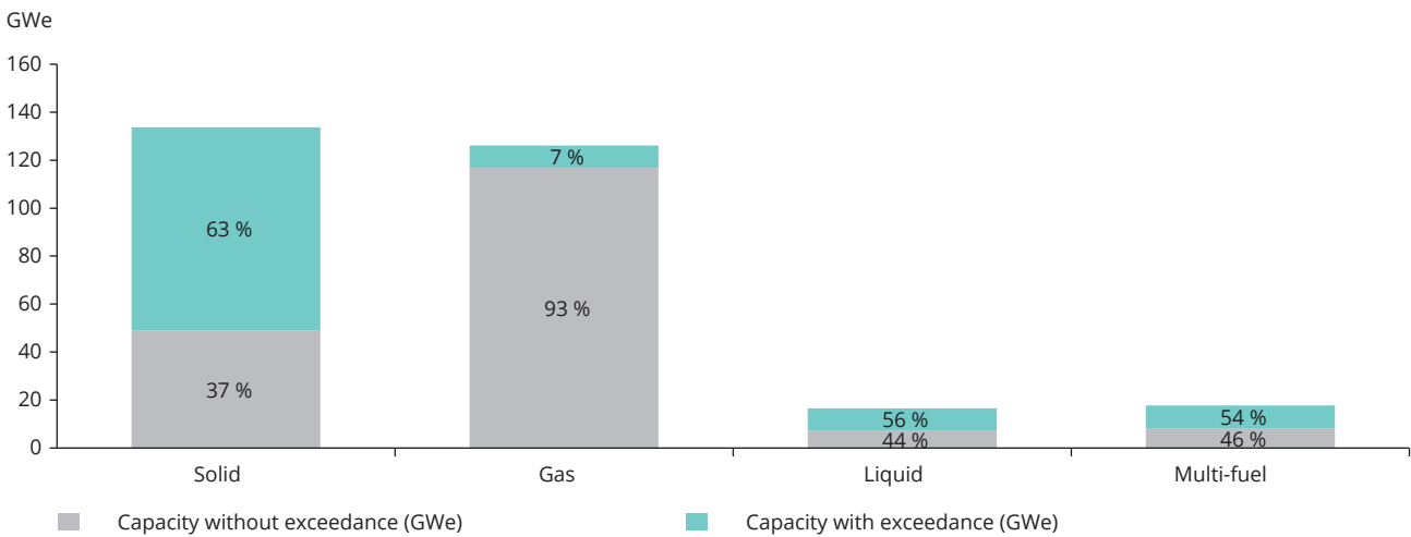
Figure 3.7 IED ELV exceedances in installed capacity by fuel type (GWe and % share)
