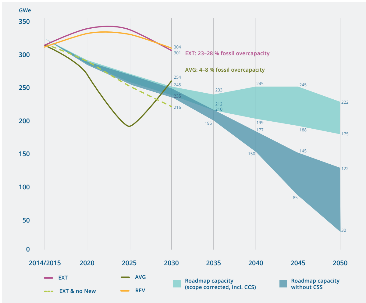
Figure ES.1 Illustrative sector capacity profiles and cost-effective capacity levels from the Energy Roadmap 2050 scenarios
