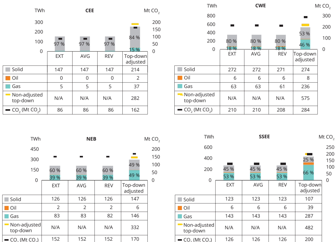
Figure 2.10 Comparison of current regional electricity generation profiles by fuel type (TWh) and carbon dioxide emissions (Mt CO 2 ), 2014/2015
