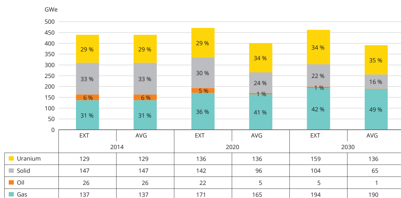
Figure A1.3 Total installed capacity in the EU-28 (GWe)
