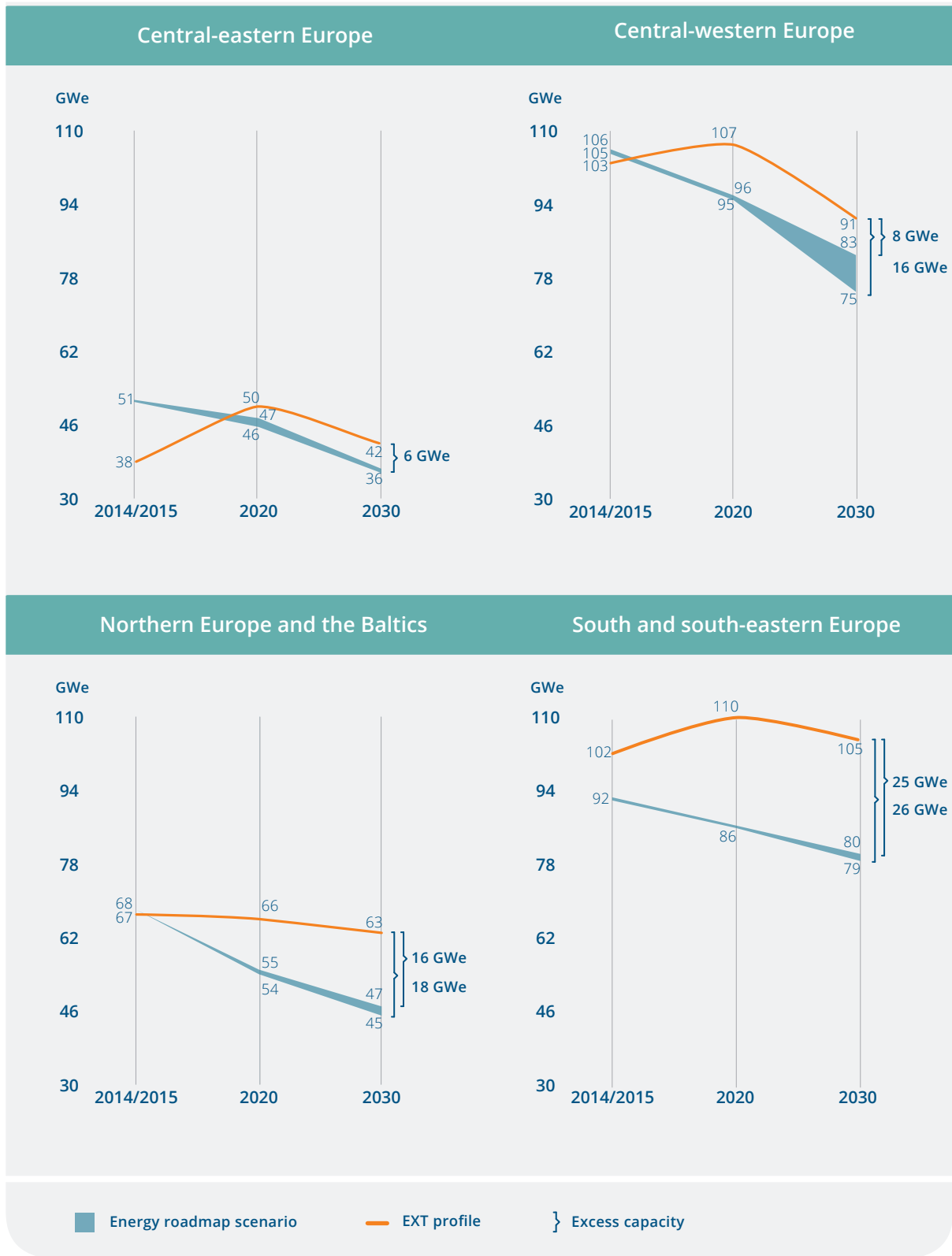
Figure 4.6 Illustrative regional fossil fuel capacity profiles (EXT) and cost-effective capacity levels (Energy Roadmap 2050)
