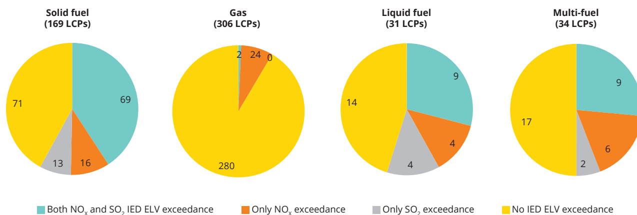
Figure 3.4 IED ELV exceedances by fuel type (number of LCPs)
