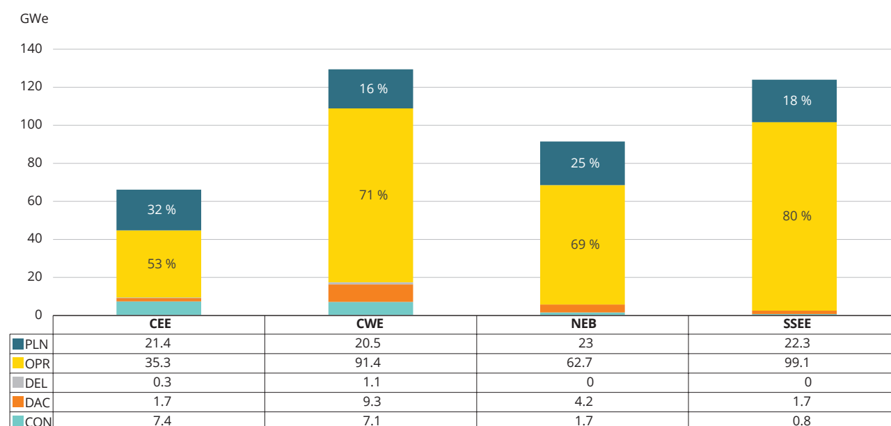
Figure 2.3 Total expected regional capacity profile by status (fossil fuel units ≥ 200 MWe)
