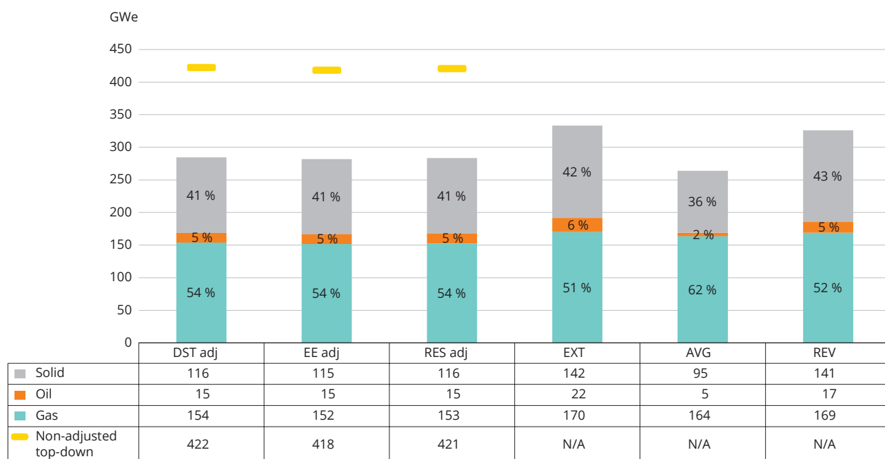
Figure 4.1 Comparison of 2020 installed capacity across the Roadmap scenarios and bottom-up profiles in the EU-27 (GWe), by fuel type
