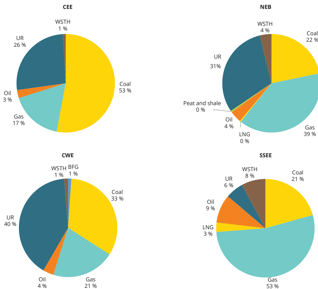
Figure 2.2 Total expected regional capacity profile, by fuel type, EU-28 (fossil fuel units ≥ 200 MWe and nuclear power)
