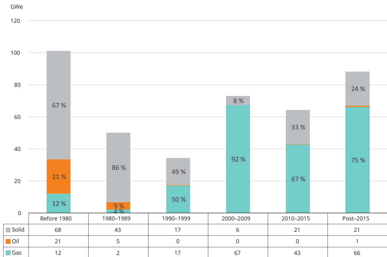
Figure 2.5 Total expected capacity by year of construction and fossil fuel type (fossil fuel units ≥ 200 MWe)
