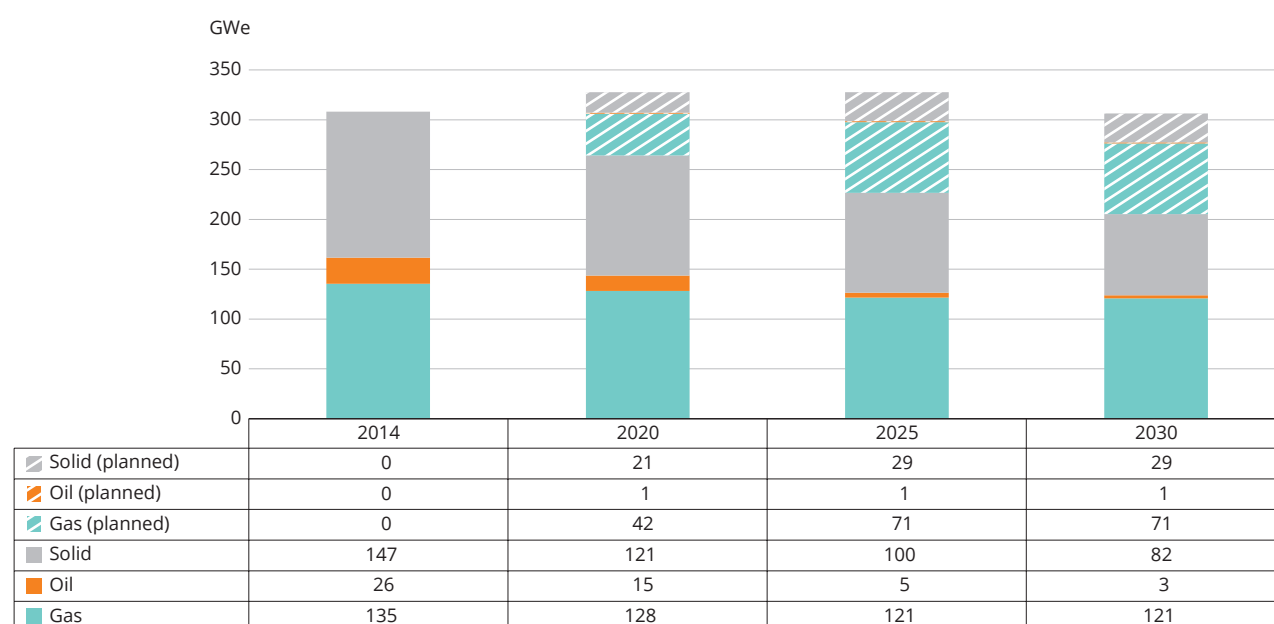
Figure 3.1 Installed capacity in the EU-28 by fuel type (GWe)
