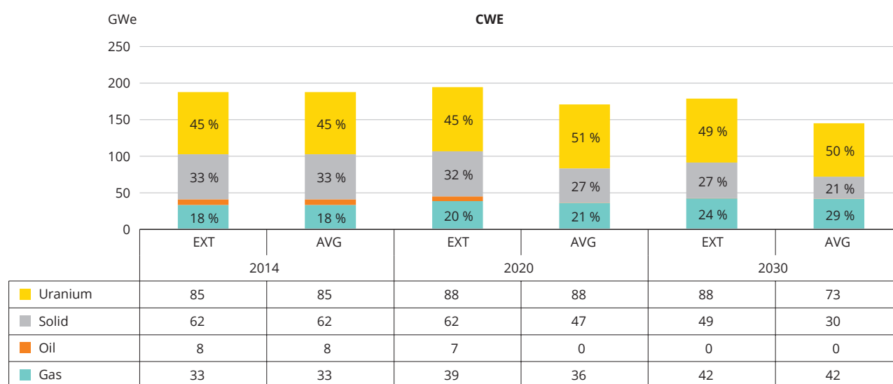
Figure A1.5 Installed capacity in central-western Europe (GWe)
