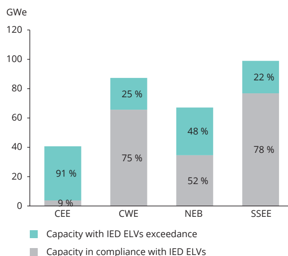
Figure 3.6 Installed capacity with and without IED ELV exceedances, by region
