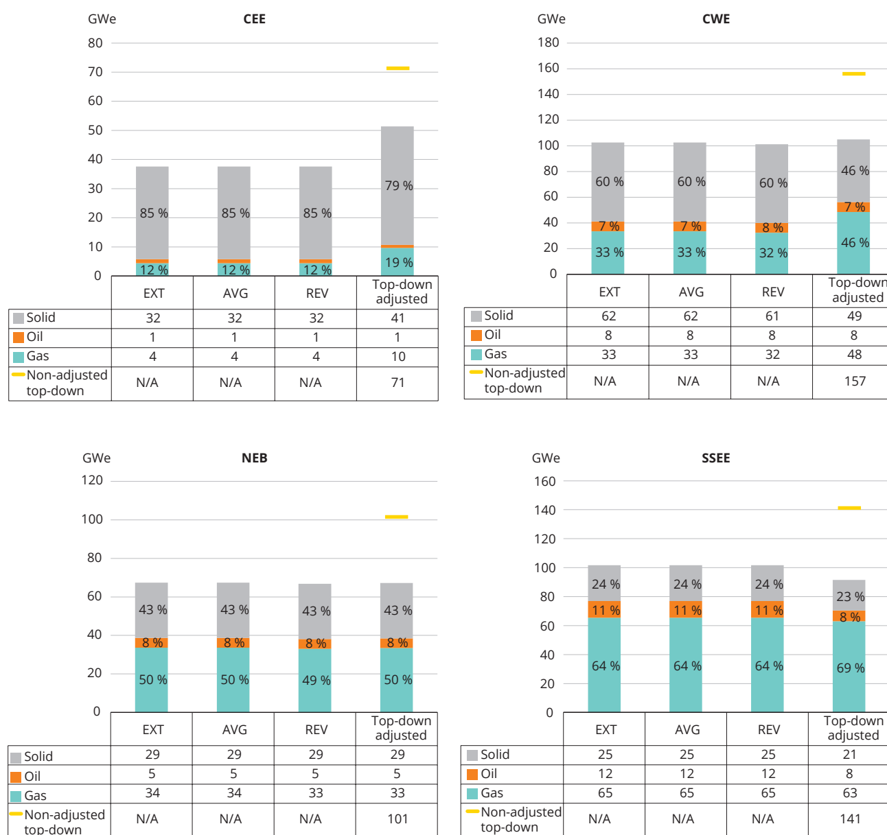
Figure 2.8 Comparison of currently installed regional capacity profiles, 2014/2015, by fuel type (GWe)
