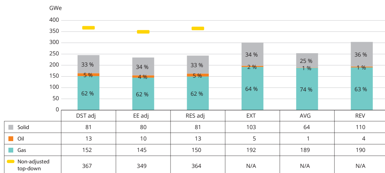
Figure 4.3 Comparison of 2030 installed capacity across the Roadmap scenarios and bottom-up profiles in the EU-27 (GWe), by fuel type
