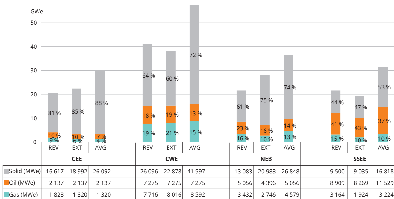
Figure 3.8 Decommissioning of regional capacity (due to EXT and REV lifetimes) from 2015 to 2030
