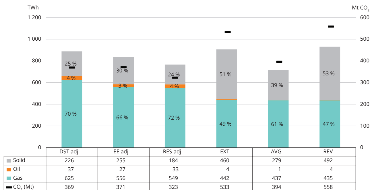
Figure 4.5 Comparison of 2030 power generation and carbon dioxide emissions (TWh/Mt CO 2 ) across Roadmap scenarios and bottom-up profiles in the EU-27, by fuel type
