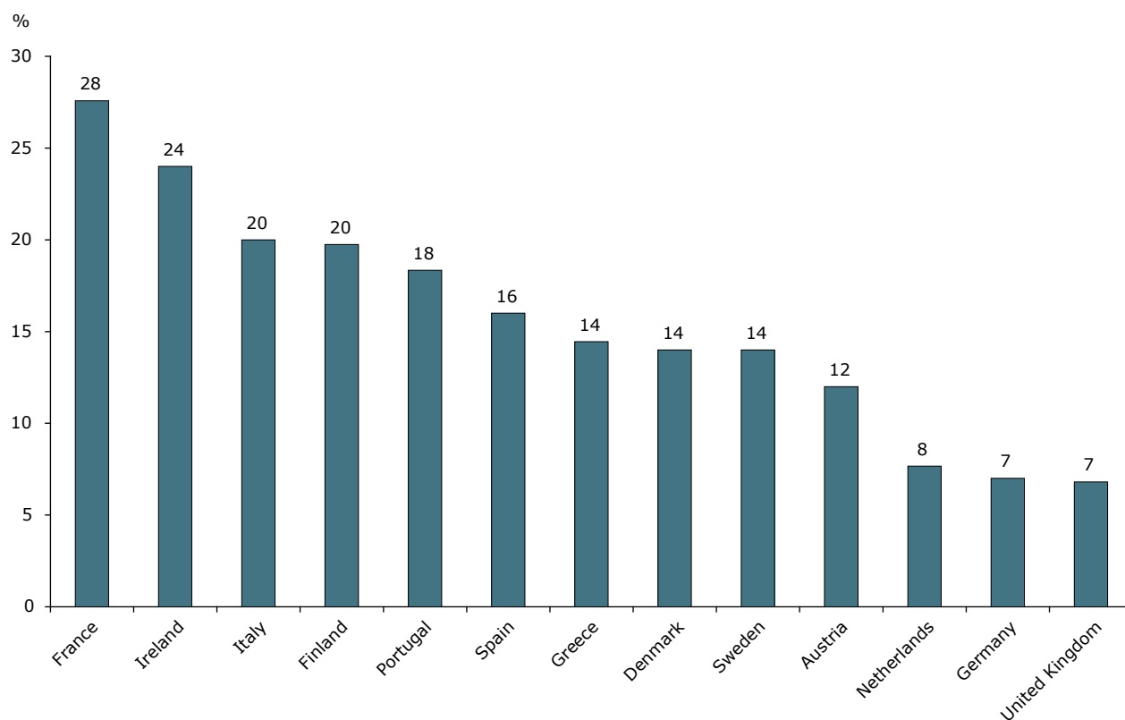
Figure 8.6 Fraction of DOC in MSW
