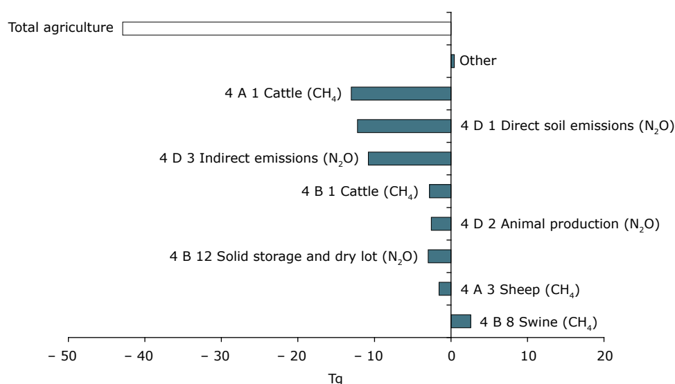
Figure 6.2 Absolute change of GHG emissions by large key source categories 1990–2004 in CO 2 equivalents (Tg) in CRF Sector 4: 'Agriculture'
