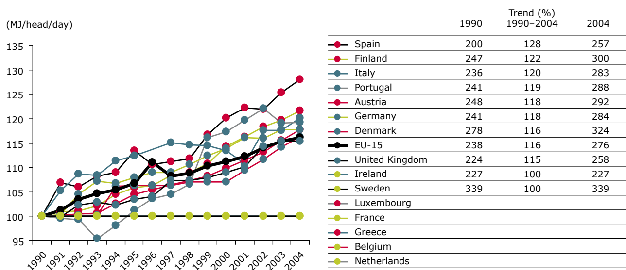
Figure 6.6 Trend of activity data for dairy cattle: average gross energy intake (GE)
