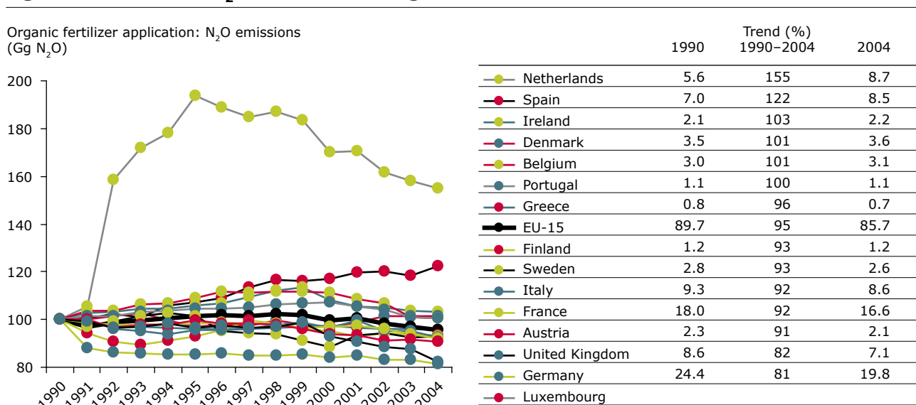
Figure 6.20 Trend of N 2 O emissions for organic fertilizer
