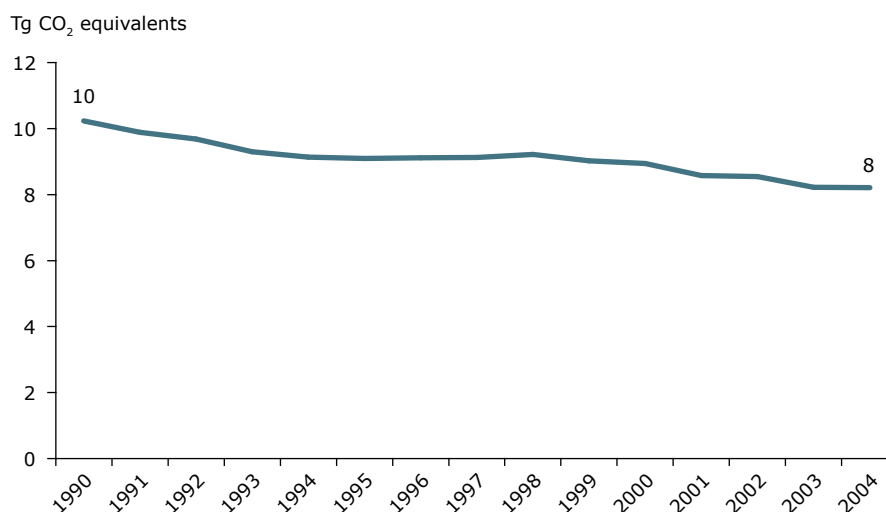
Figure 5.1 EU-15 GHG emissions for 1990–2004 from CRF Sector 3: 'Solvent and other product use' in CO 2 equivalents (Tg)
