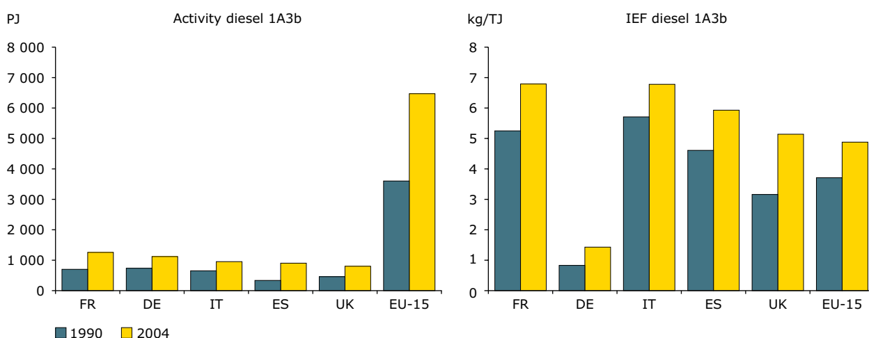
Figure 3.52 Activity data and implied emission factor for N 2 O emission from diesel oil in 1.A.3.b
