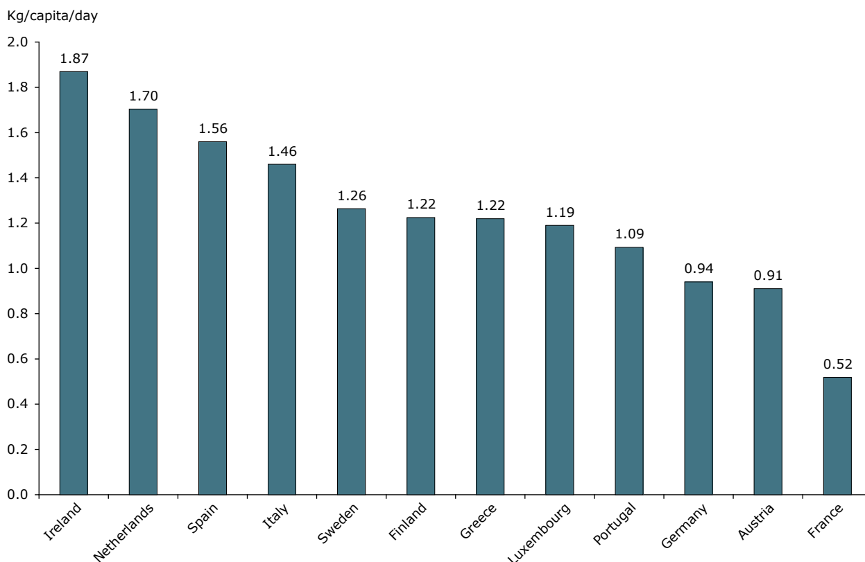
Figure 8.3 Waste generation rate
