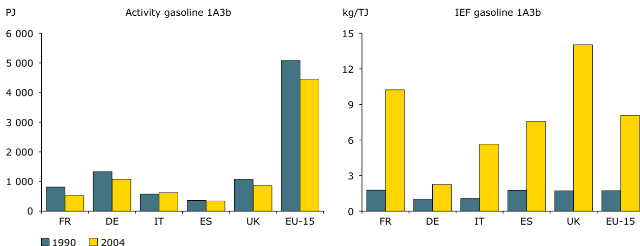
Figure 3.53 Activity data and implied emission factors for N 2 O from gasoline 1.A.3.b
