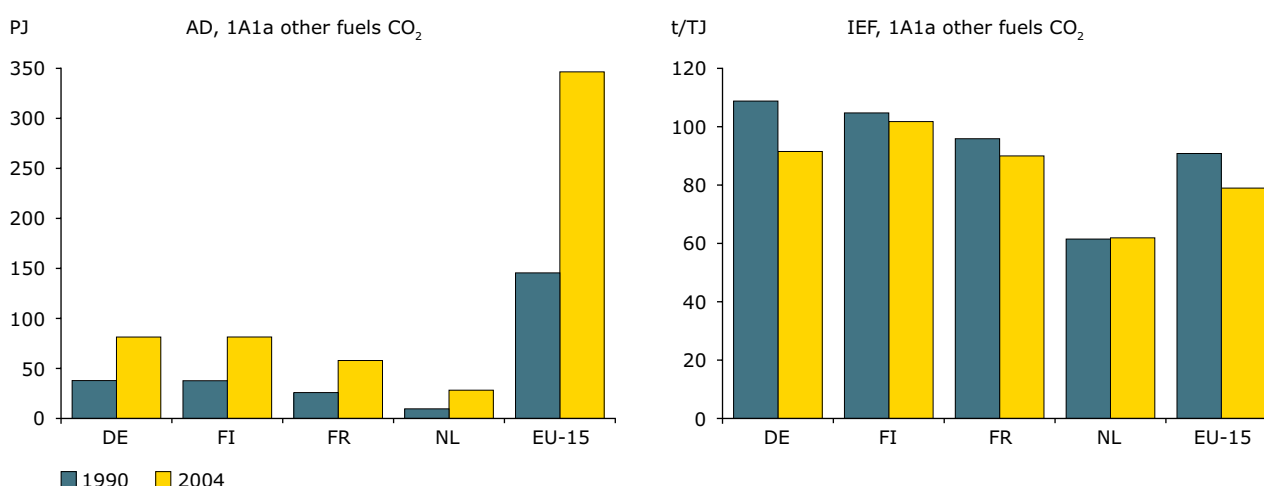
Figure 3.9 Activity data and implied emission factors for CO 2 from other fuels in 1A1a
