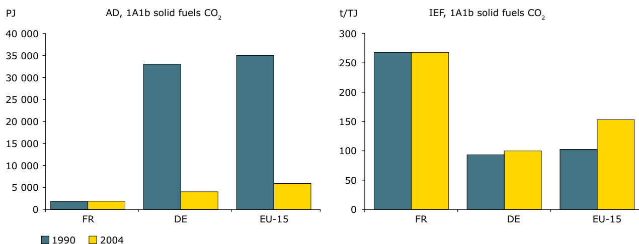
Figure 3.12 Activity data and implied emission factors for CO 2 from solid fuels in 1A1b
