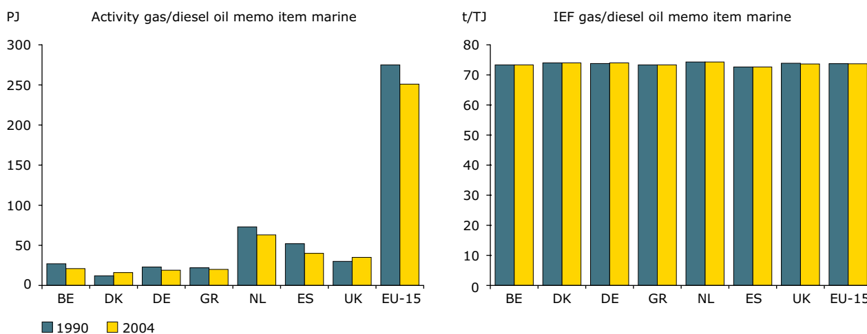
Figure 3.90 Activity data and implied emission factors for CO 2 from 'Marine bunkers' – gas/diesel oil
