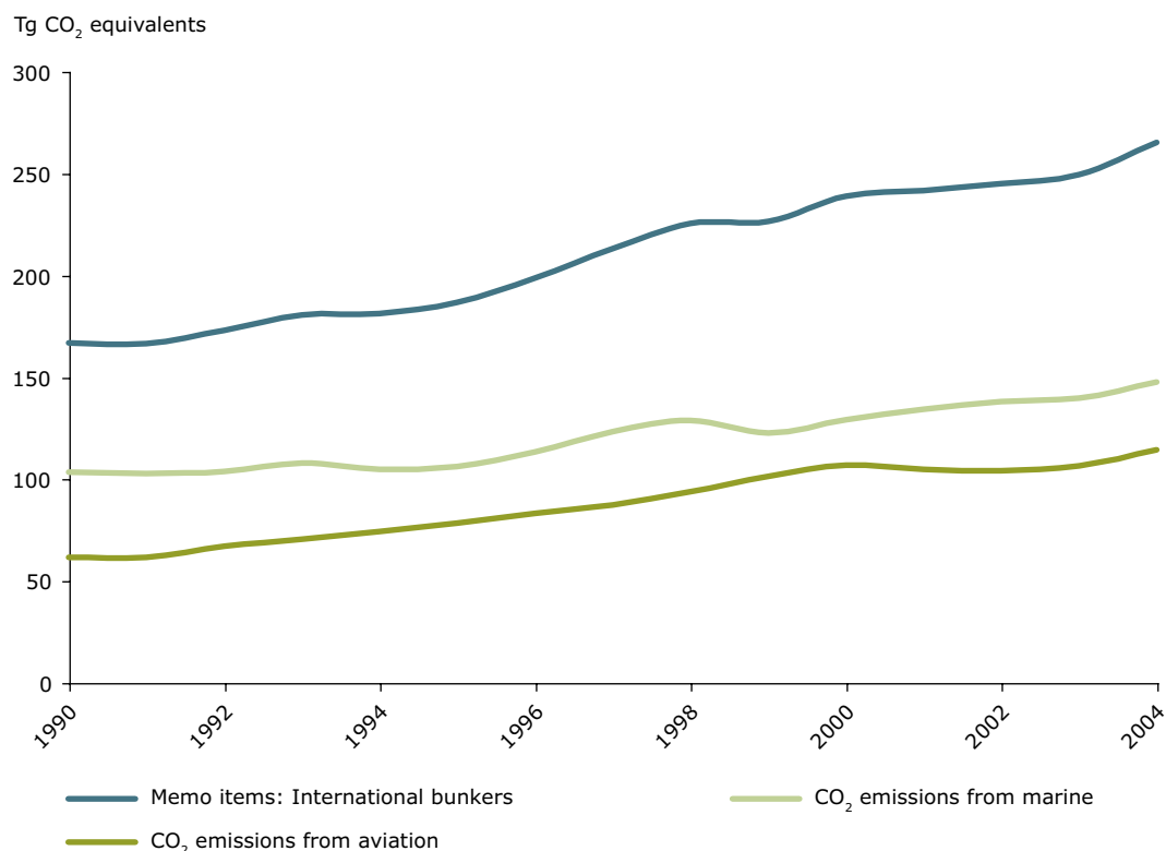
Figure 3.86 CO 2 Aviation bunkers
