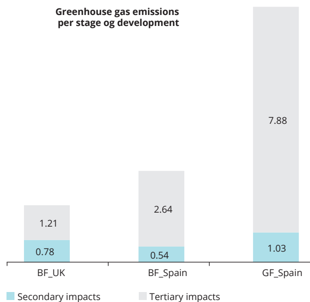
Figure 3.9 Contribution of each stage of development to GHG emissions (t CO 2 eq) across the three case studies (20-year lifespan, functional unit 1 m 2 of built surface)
