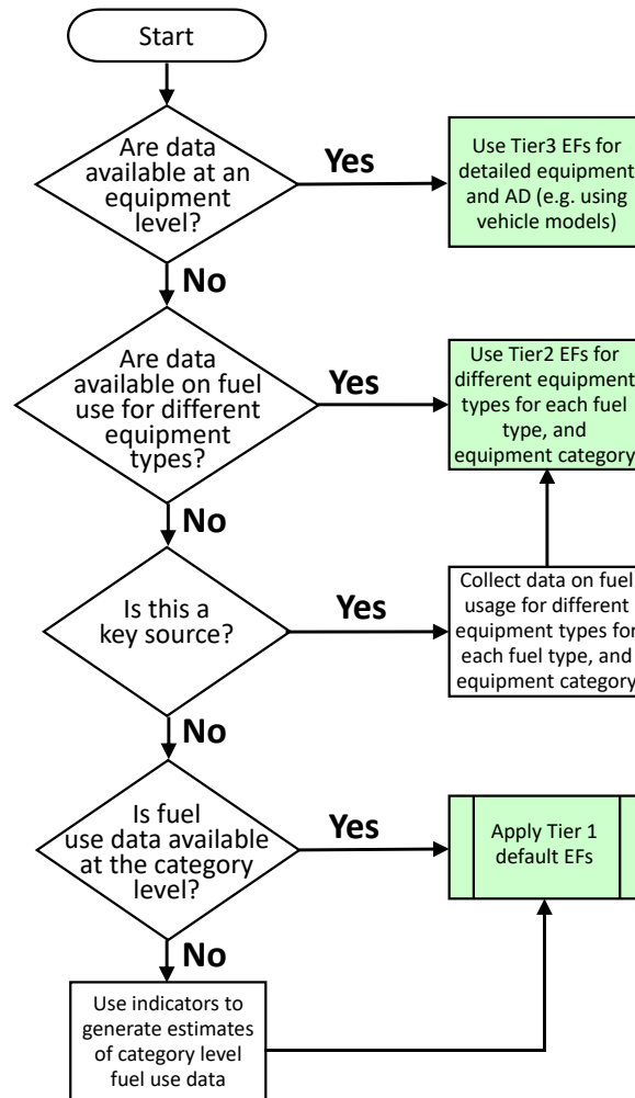
Figure 3-1 Decision tree for other off-road mobile machinery
