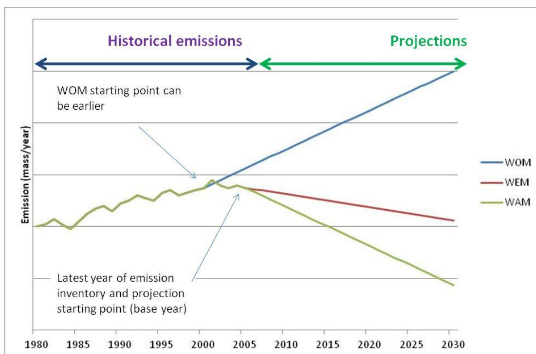
Figure 2-1 Emission projections
