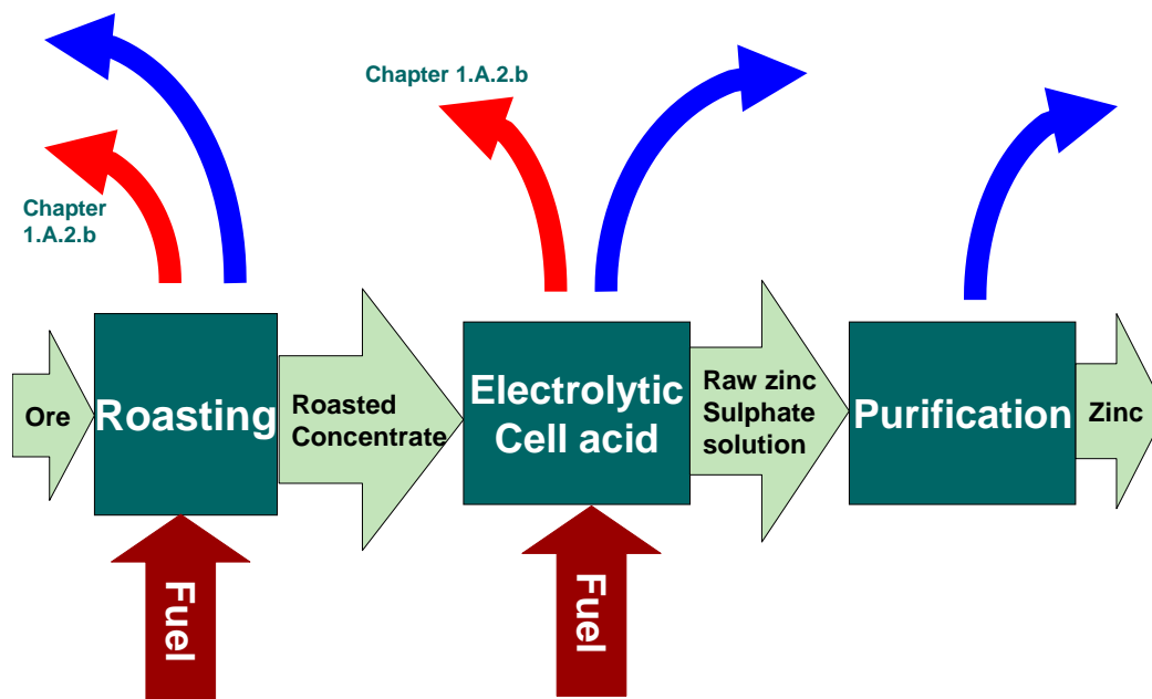
Figure 2.2 Process scheme for source category 2.C.6 Zinc production, electrochemical zinc production process
