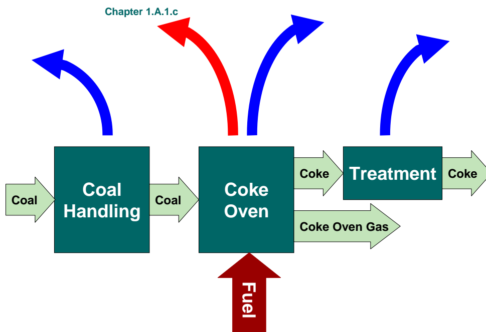
Figure 2-1 Process scheme for coke production, the most important process within source category 1.B.1.b Solid fuel transformation; combustion emissions from the coke oven are treated in chapter 1.A.1.c
