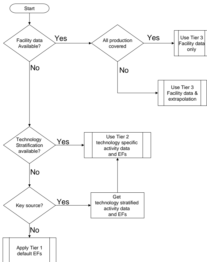
Figure 3.1 Decision tree for source category 2.D.1 Pulp and Paper
