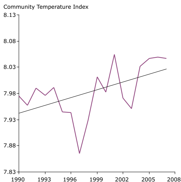
Figure 2 Community Temperature Index of butterflies
